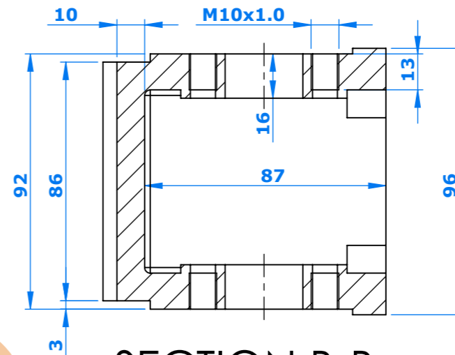
SECTION B-B SCALE 1 : 1.9
